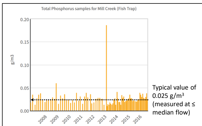
Figure 2. Total phosphorus concentrations at the Fish Trap in Mill Creek from 2007 to 2016, showing no decline in concentrations measured at or below the median flow of the creek. ORC data from LAWA website (accessed July 20, 2018).
